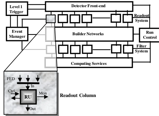
Figure 1: CMS DAQ System
