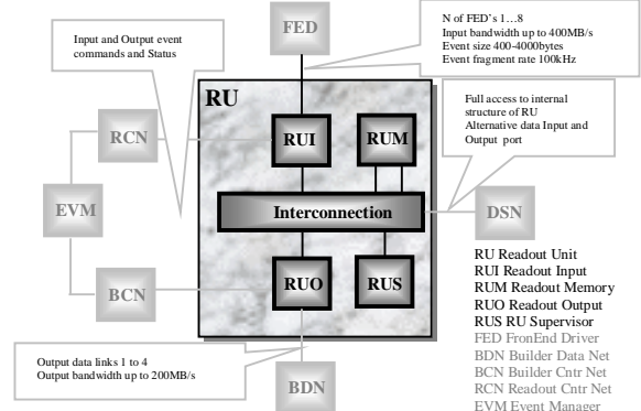
Figure 2: RU Functional Blocks
